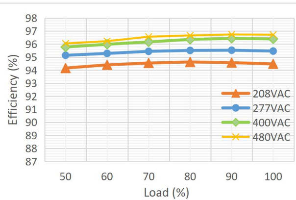
Figure 8.Efficiency vs Different Loads for CH1(1)
