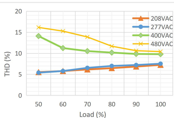
Figure 10.Total Harmonics vs Different Loads for CH1(2)
