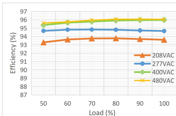
Figure 11. Efficiency vs Different Loads for CH1(2)
