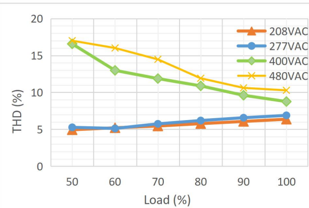
Figure 7.Total Harmonics vs Different Loads for CH1(1)
