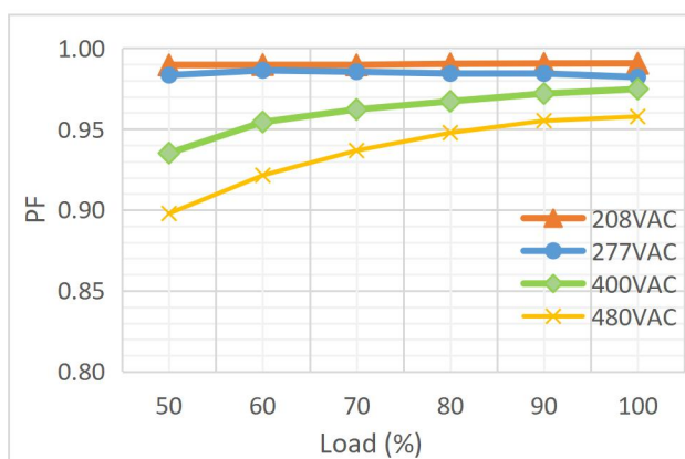
Figure 15. Power Factor vs Different Loads for CH1,CH2,CH3,CH4,CH5(1)
