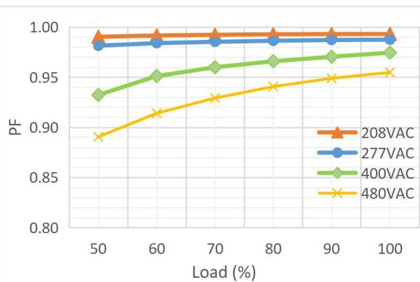
Figure 9.Power Factor vs Different Loads for CH1(1)
