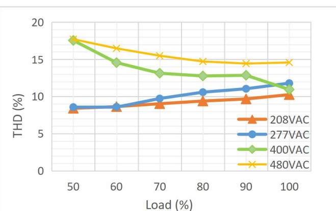
Figure 16. Total Harmonics vs Different Loads for CH1,CH2,CH3,CH4,CH5(2)
