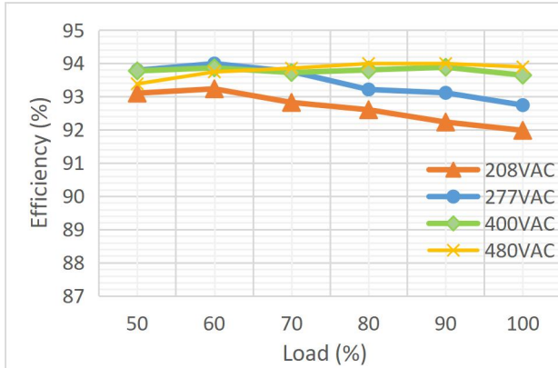
Figure 17. Efficiency vs Different Loads for CH1, CH2, CH3, CH4, CH5(2)
