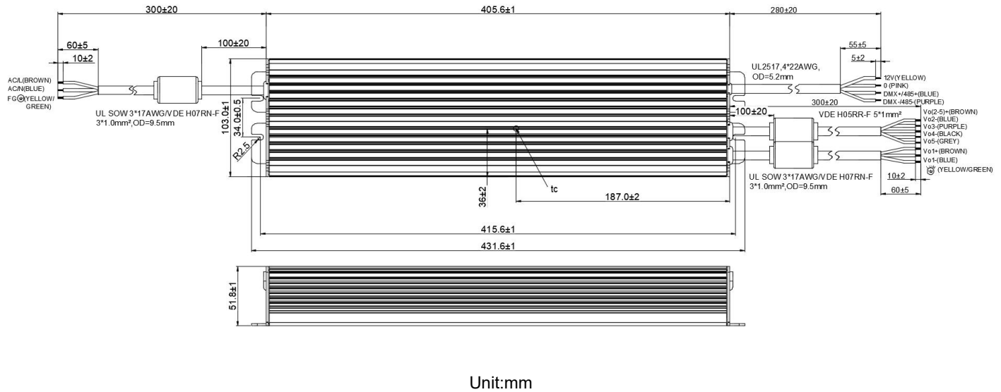
Figure 21.Mechanical Drawing
