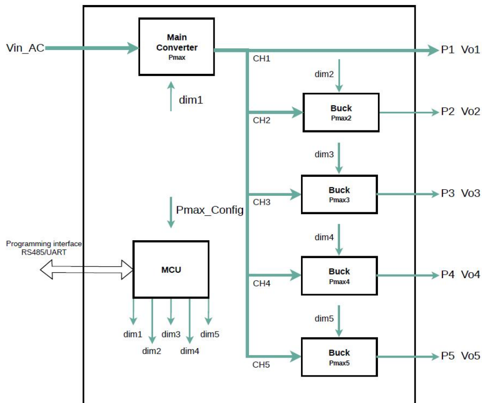
Figure 19. The Block Diagram of Automatic Power Distribution for a 5-channel LED Driver
