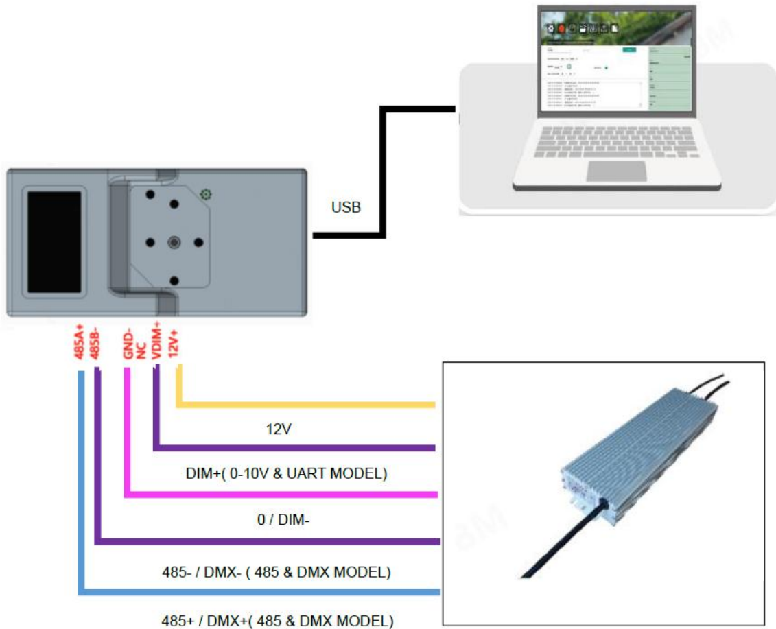
Figure 20.Programming Wiring
