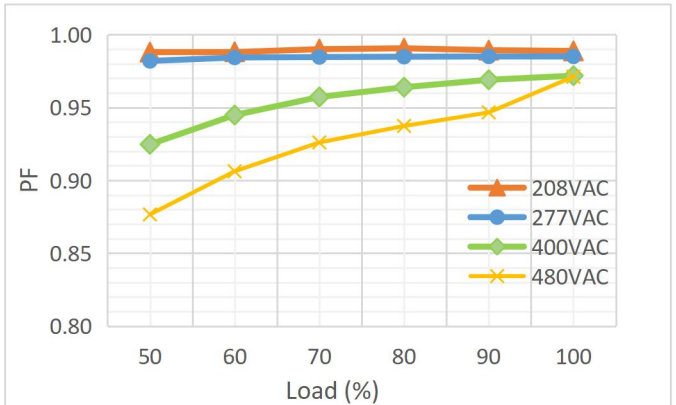
Figure 18. Power Factor vs Different Loads for CH1, CH2, CH3, CH4, CH5(2)
