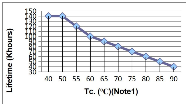
Lifetime vs Case Temp
