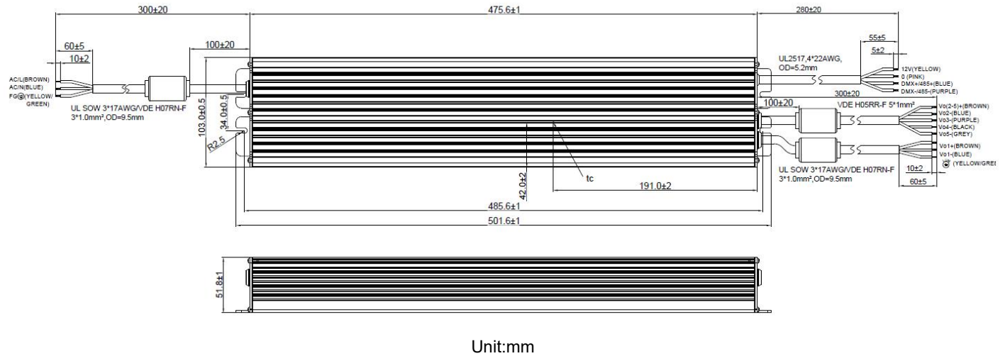
Figure 18. Mechanical Drawing
