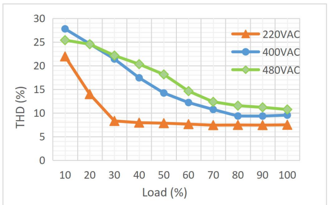
Figure 10. Total Harmonics vs Different Loads for CH1(1600HTH400CV)
